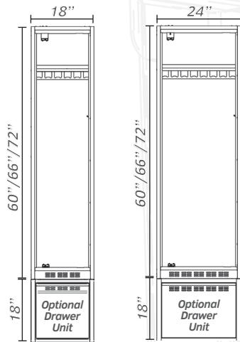
FRONT VIEW - BASIC CONFIGURATION
